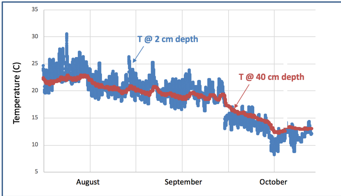
Figure 4: Three months of soil temperature data at 2cm and 40cm, Ithaca, NY.
